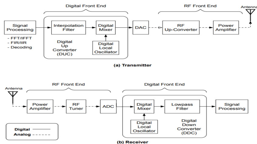
Figure 1 (Generalized SDR architecture) (Akeela & Dezfouli, 2018)
